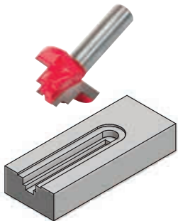
Flush Bolt Router Cutter
